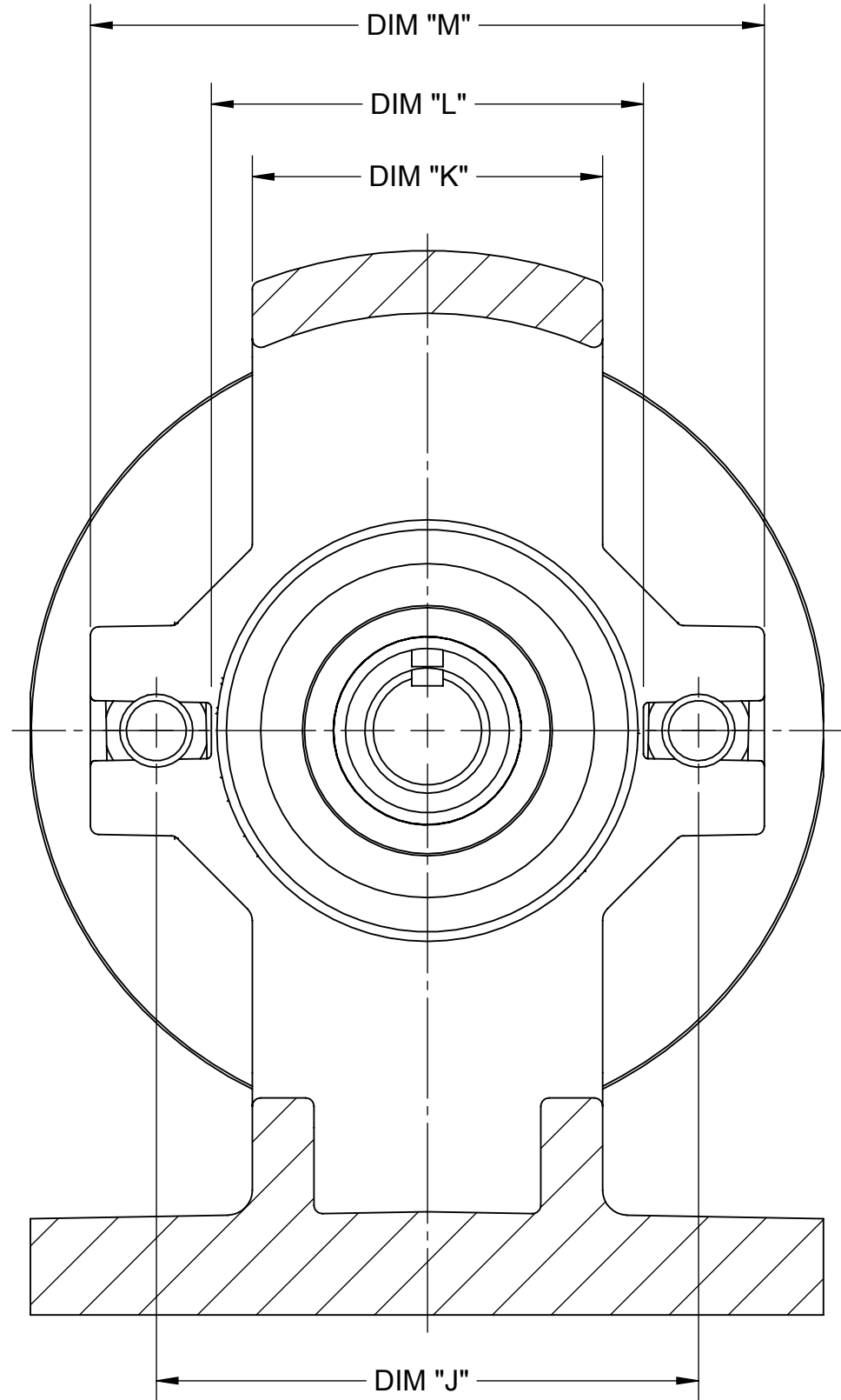
SECTION B-B
