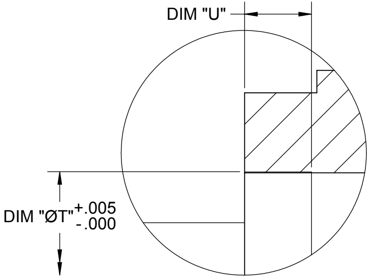
DETAIL A SCALE_4 : 1 APPLIES TO MODELS G1-24/32, G1-55/69 ONLY
